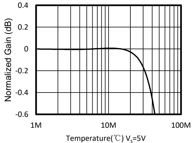
AC Response
